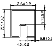
TUBE MECHANICAL DIMENSION
