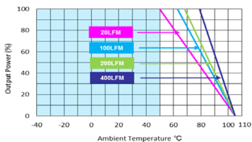
MJWI25-24S05, MJWI25-24S12, MJWI25-24D12, MJWI25-24D15, MJWI25-48D12, MJWI25-48D15 Derating Curve without Heatsink
