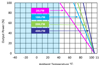
MTQZ75-72S05, MTQZ75-110S05 Derating Curve with Heatsink
